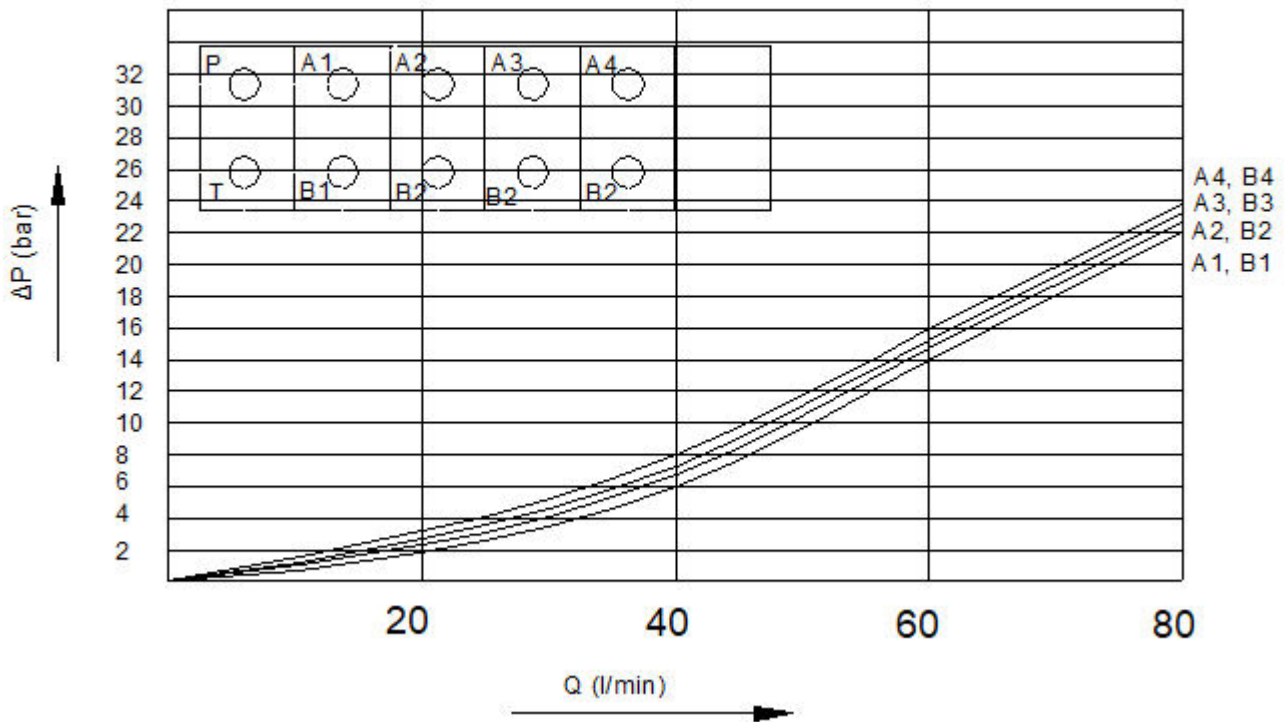
Pressure drop A/B > T1
