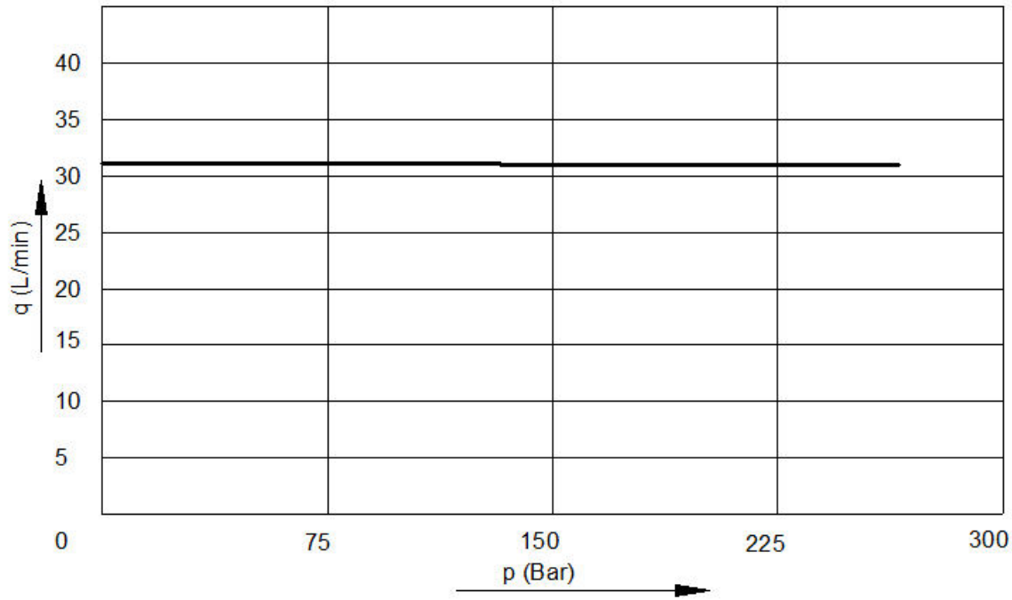
p-q curve
